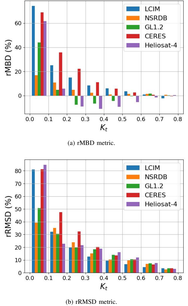
Fig. 7. Performance metrics on cloudiness bands (spatially averaged).
