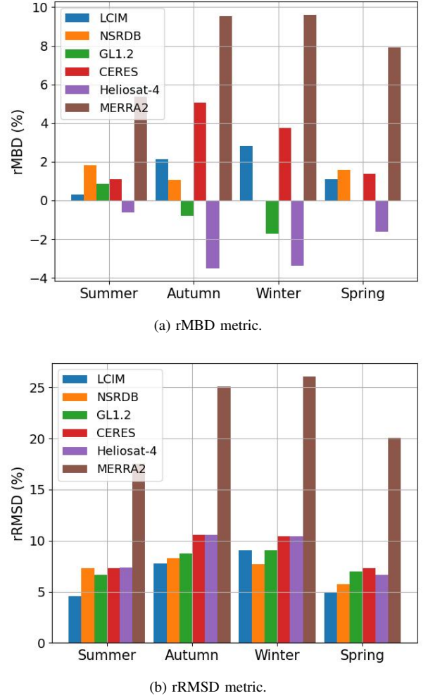
Fig. 5. Performance metrics in each season. The measurement's mean in \text{kWh/m}^2 are: 6.7 (summer), 3.3 (autumn), 3.2 (winter) and 6.5 (spring).
